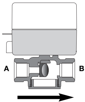
2-way valve normally closed actuator
