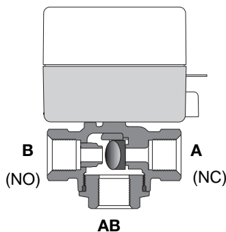
3-way valve normally closed actuator (Note: 3-way uses only normally closed actuator)
